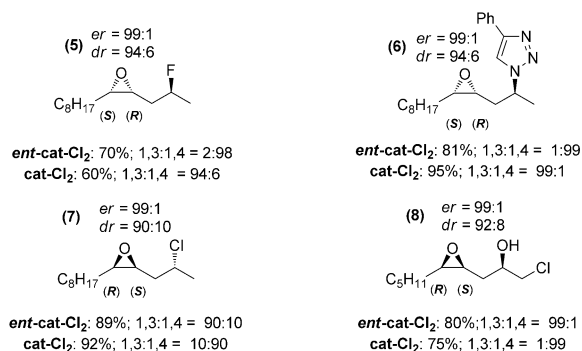
Scheme 4. REOs of various \beta -epoxy functionalized substrates (7 mol % cat., 1.5 equiv Lut-HCl, 1.5 equiv Mn, 2.2 equiv Bu 3 SnH, 0.3 M in THF, 3 days, 25 °C).
